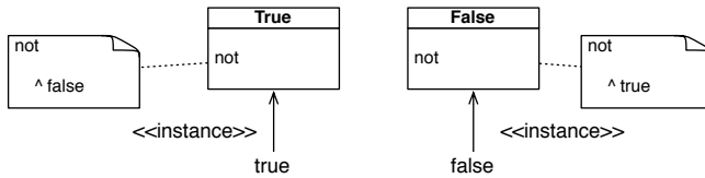
Figure 13-3 Two methods for one message each one returning the other instance.
