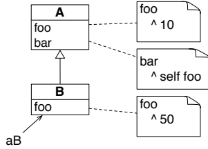
Figure 14-9 Self semantics abstractly explained.
