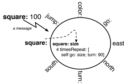
Figure 8-1 An object presents to the other objects an interface composed of a set of messages defining what he can do. This behavior is realized by methods that specify how the behavior is implemented. When a message is sent to an object a method with the message name (called selector) is looked up and executed.
