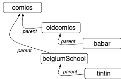
Figure 9-5 A graph of objects to represent our file system.
