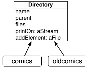
Figure 9-3 The Directory class and some instances (directories).
