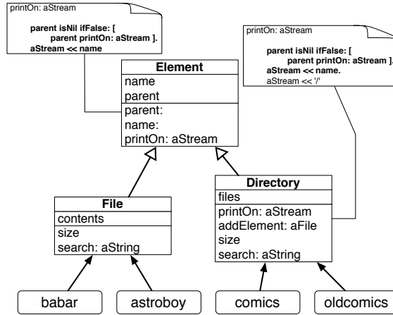
Figure 15-2 Improving the logic (but not fully).
