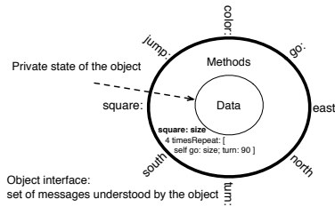
Figure 8-3 A turtle is an object which has an interface, i.e., a set of messages to which it can reply and a private state that only its methods can access.
