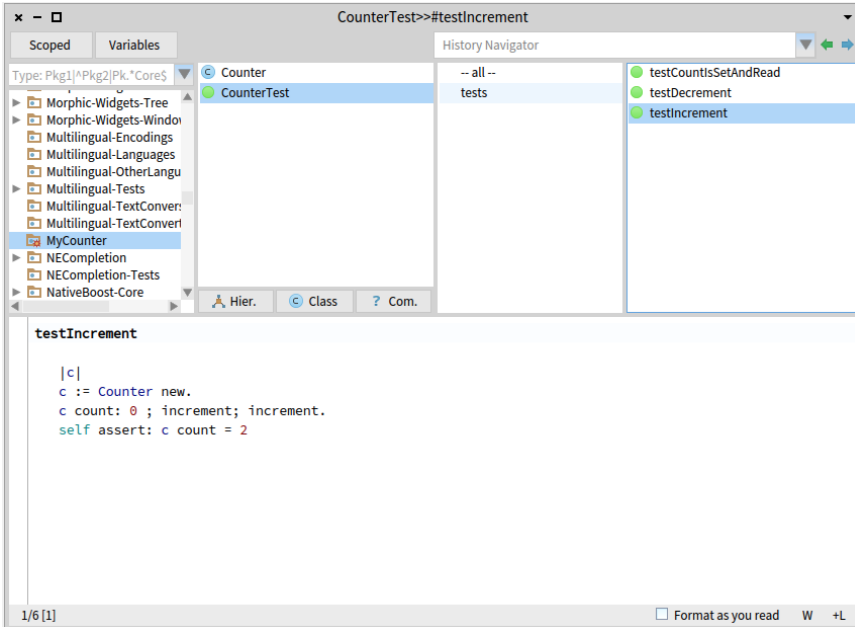
Figure 5-5 Class with green tests.
