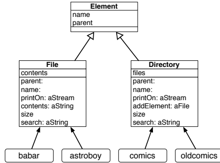
Figure 14-5 State factored between the two classes and their superclass.
