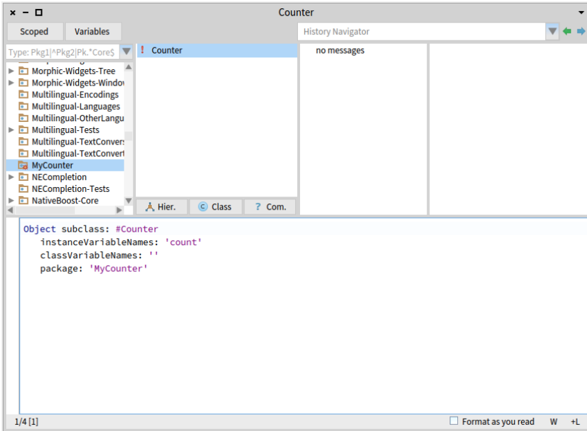
Figure 5-2 Class created.
