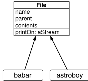
Figure 9-6 A new class and its instances.
