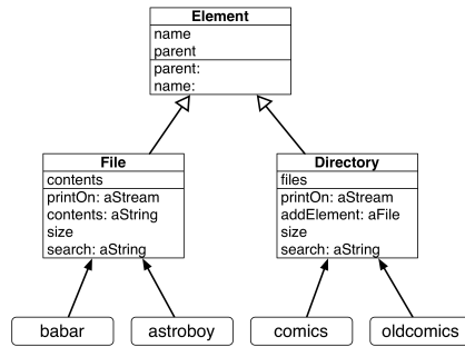
Figure 14-6 State and Methods factored out in the superclass.
