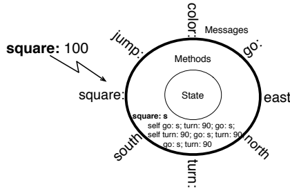
Figure 8-2 The message square: can be implemented differently. This different implementation does not impact the sender of the message who is not concerned by the internals of the object.
