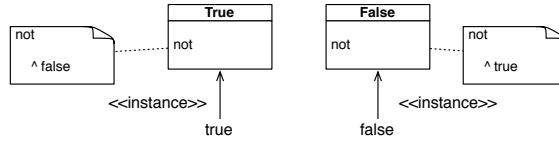
Figure 13-2 Two methods for one message.
