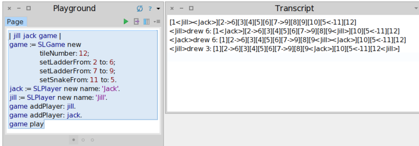
Figure 18-11 Automated play.
