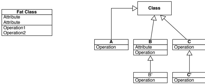
Figure 13-7 One single class vs. a nice hierarchy.
