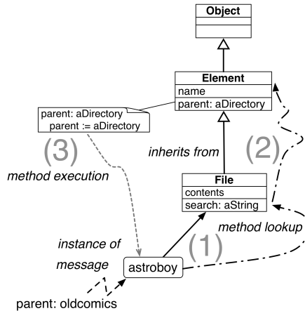
Figure 14-7 When an object receives a message, the corresponding method is looked up in its class and if necessary its superclasses (Step 1 and 2). Then the method is executed on the message receiver (Step 3).
