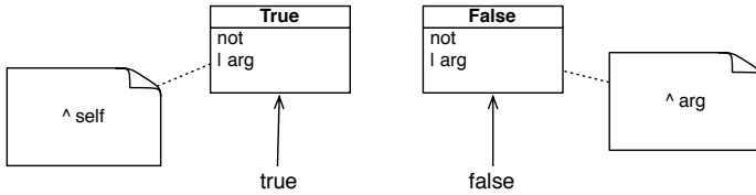
Figure 13-5 Disjunction implementation: two methods.
