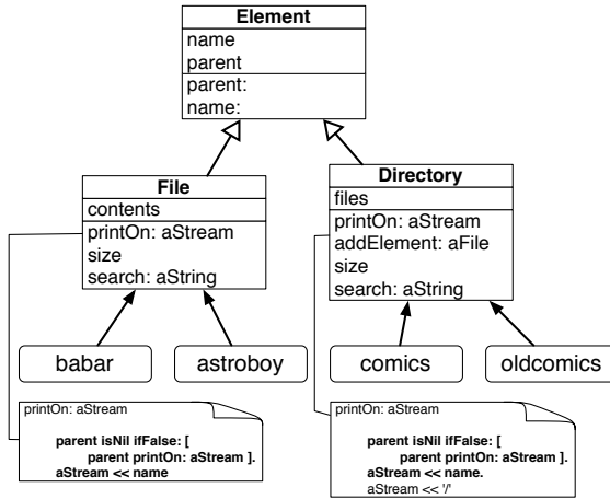
Figure 15-1 MFFile and MFDirectory contain duplicated logic in printOn:.
