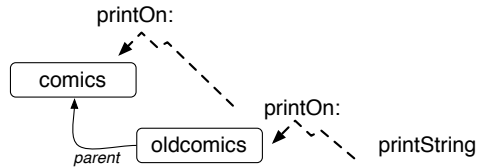
Figure 9-4 Navigating an object graph by sending message to different objects.
