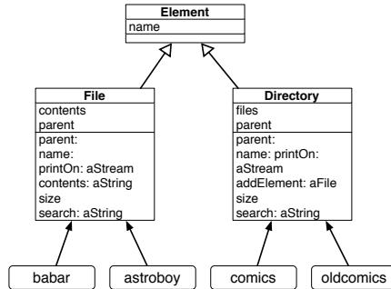
Figure 14-3 Moving the instance variable name to the superclass.
