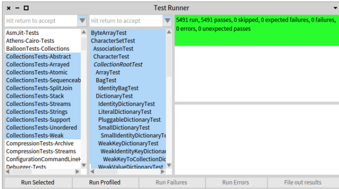
Figure 6-2 Running SUnit tests using the TestRunner .
