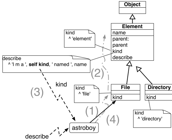
Figure 14-8 A self-send creates a hook (kind) that subclasses override. The method describe is called a template because it creates a context.
