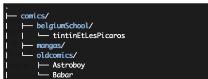
Figure 9-1 Some directories and files organised in a file system.
