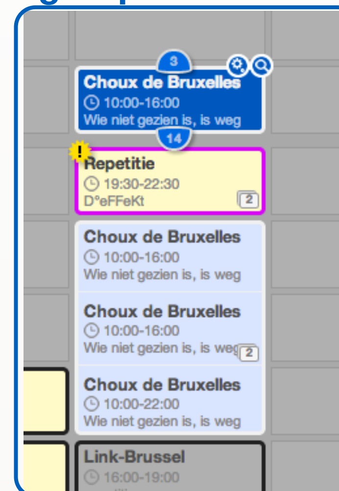
group visualization
