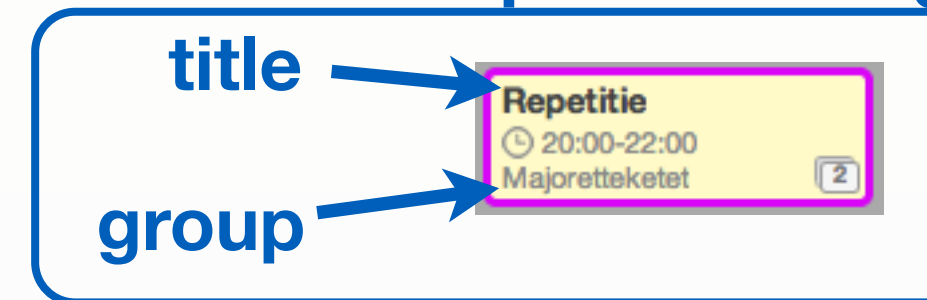
in-place editing
